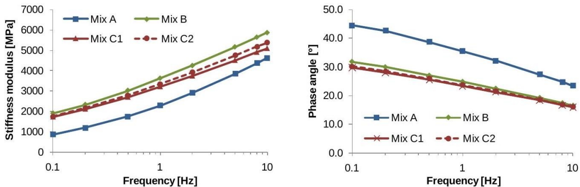
Fig. 6 - Stiffness modulus and phase angle results of the studied mixtures
